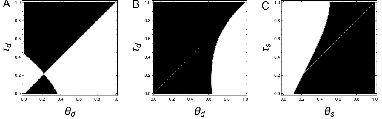
Figure 2: Pairwise invasibility plots. Panel A displays the difference \widetilde{W}(\tau_d, \theta_d, 1) - \widetilde{W}(\theta_d, \theta_d, 1) for all combinations of \theta_d ( x -axis) and \tau_d ( y -axis) values (and thus holding \theta_s = 1 fixed), for the parameter values a = 0.1 , b = -0.5 and c = 1 of the linear quadratic game (44) ( \widetilde{W}(\tau_d, \theta_d, 1) is thus defined by (60)). The difference is zero on the diagonal, since \tau_d = \theta_d . The black region depicts all the combinations (\theta_d, \tau_d) such that the difference is negative, while the white region outside the diagonal depicts all the combinations (\theta_d, \tau_d) such that the difference is strictly positive. The candidate given by eq. (62) is \theta_d^* \approx 0.22 , which the graph shows is uninvadable. Panel B displays the difference W(\tau, \theta) - W(\theta, \theta) determined by eqs. (54)–(59) of a mutant \tau = (\tau_d, 1) in a resident \theta = (\theta_d, 1) population for all combinations of resident \theta_d ( x -axis) and mutant \tau_d ( y -axis) trait values (and thus holding \theta_s = 1 and \tau_s = 1 fixed) for the parameter values a = 0.1 , b = -0.5 and c = 1 of the linear quadratic game (44). On the diagonal, the difference equals zero (and invasion fitness equals one) since \tau_d = \theta_d . The black region depicts all combinations (\theta_d, \tau_d) such that the difference is negative, i.e., W(\tau, \theta) < 1 , so that the mutant \tau_d cannot invade, while the white region outside the diagonal depicts all combinations (\theta_d, \tau_d) such that the difference is positive, W(\tau, \theta) > 1 , so that the mutant can invade. The graph thus shows that all values of (\theta_d, 1) with \theta_d below approximately 0.6 are uninvadable. There is thus a multiplicity of uninvadable types, which necessarily contains that of Panel A. Note that resident values above approximately \theta_d \approx 0.9 are invadable by any mutation \tau_d < \theta_d , while resident values between approximately 0.6 and 0.9 are invadable by mutants with \tau_d = \theta_d - \delta for \delta > 0 large enough. Panel C displays W(\tau, \theta) - W(\theta, \theta) determined by eqs. (54)–(59) for a mutant \tau = (\tau_d, \tau_s) in a resident \theta = (\theta_d, \theta_s) population for all combinations of resident \theta_s ( x -axis) and mutant \tau_s ( y -axis) trait values holding \tau_d = \theta_d = \tilde{\rho}(\theta_d) fixed and given by (61) under the parameter values a = 0.1 , b = -0.5 and c = 1 of the linear quadratic game (44). As for Panel B, the black region depicts all combinations (\theta_s, \tau_s) such that the difference is negative, i.e., W(\tau, \theta) < 1 , so that the mutant \tau_s cannot invade, while the white region outside the diagonal depicts all combinations (\theta_s, \tau_s) such that the difference is positive, W(\tau, \theta) > 1 , so that the mutant can invade. The graph thus shows that all values of (\theta_s, \tilde{\rho}(\theta_d^*)) with \theta_s above approximately 0.5 are uninvadable.
