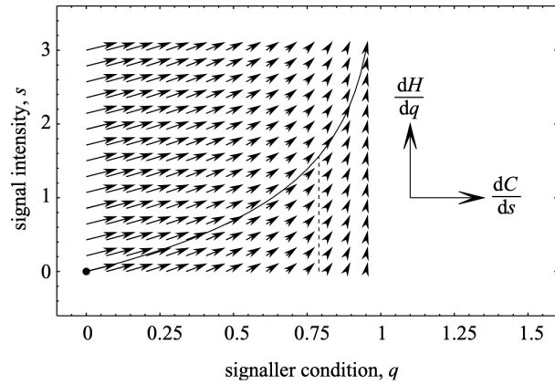
Figure 2. The vector field V(s,q) for the game treated in example 2.1. Each vector has magnitude (d/dq) H(q', R_q^*(q))|_{q=q'} direction and (d/ds) C(q',s)|_{s=s'} in the horizontal direction. The solid curve is the equilibrium signalling strategy S(q) .
