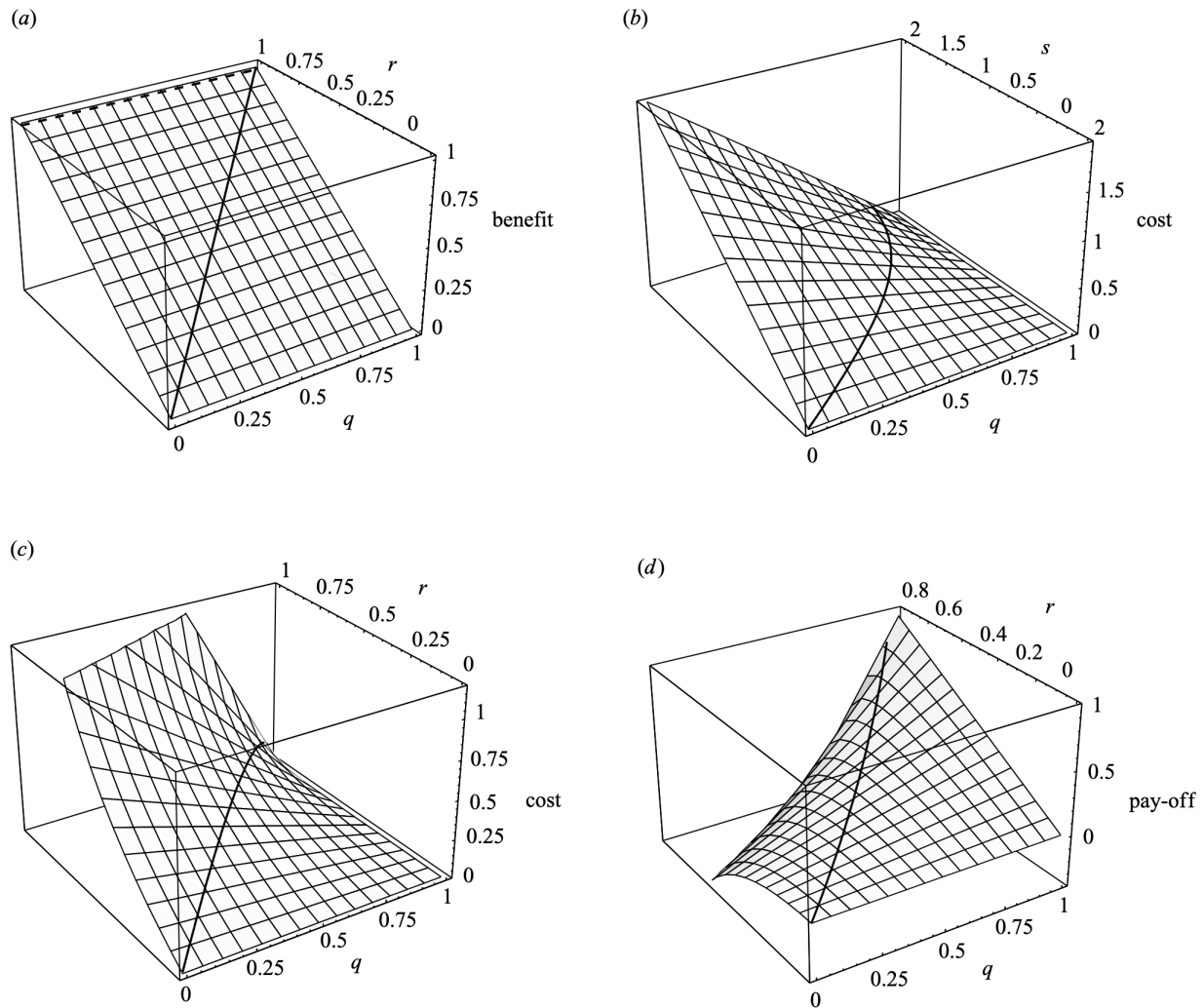
Figure 1. Benefit, cost and net fitness functions for example 2.1. The separating equilibrium is represented by the dark curves across the surfaces. (a) Benefit function H(q, r) : dashed line, signaller's desired response; solid line, receiver's desired response; (b) cost C(q, s) as a function of quality and signal sent; (c) cost C_r(q, r) as a function of quality and response elicited; (d) signaller's net fitness H(q, r) - C_r(q, r) .
