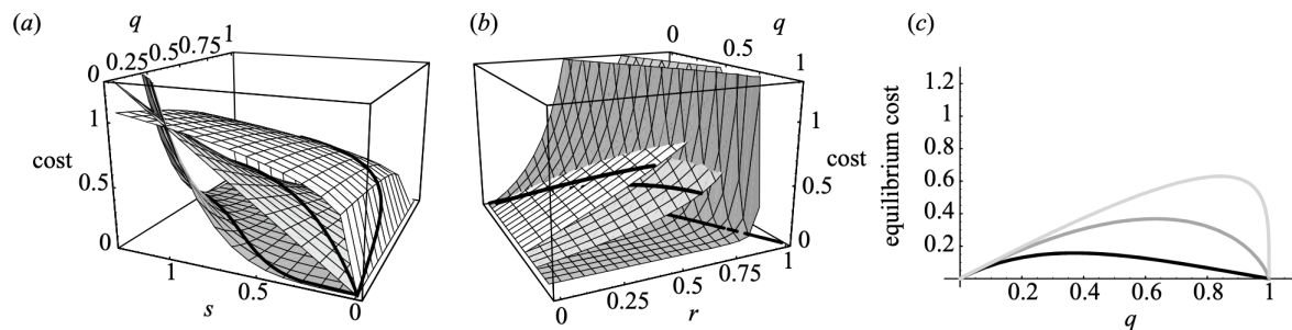
Figure 5. Signal costs for cost functions C(q,s) = s^\alpha(1-q)^\alpha . Light grey, \alpha = \frac{1}{3} ; medium grey, \alpha = 1 ; dark grey, \alpha = 4 . Dark curves show the equilibrium path for each cost function. (a) Cost of signalling, as a function of signaller's quality and signal intensity. (b) Cost of signalling, as a function of signaller's quality and response received given equilibrium behaviour by the receiver. The upper cost surfaces have been partially cut away to reveal those beneath them. (c) Signal cost at equilibrium, as a function of signaller quality.
